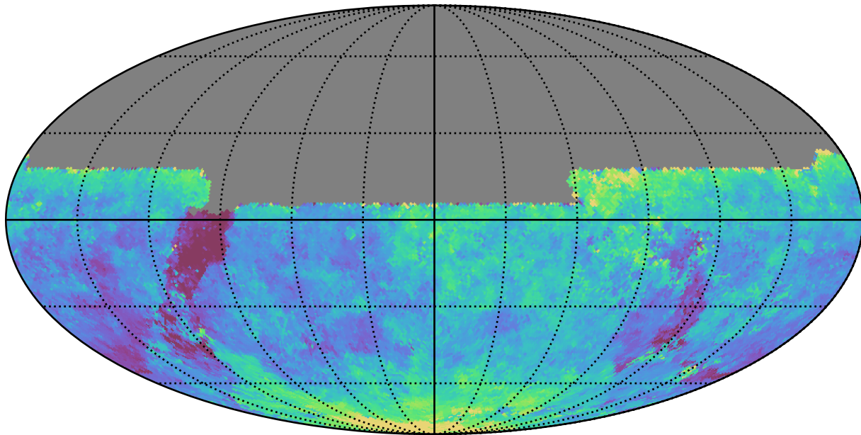
weather_cloudso31v3.4_10yrs All sky u band: Median seeingEff
