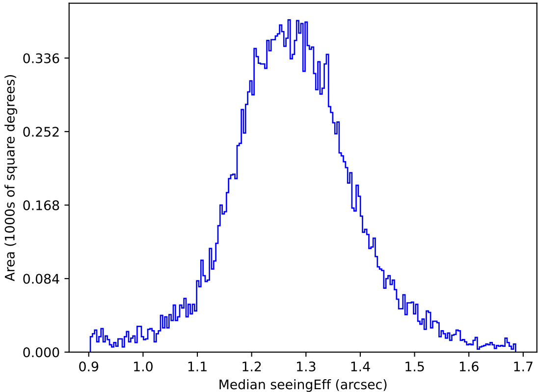
weather_cloudso31v3.4_10yrs All sky u band: Median seeingEff
