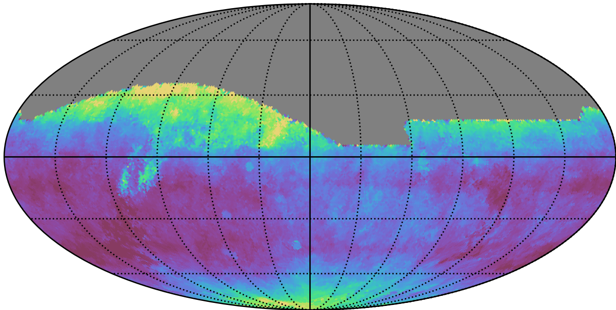
weather_cloudso31v3.4_10yrs All sky r band: Median seeingEff
