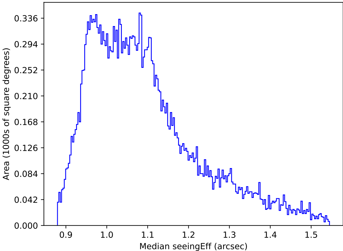
weather_cloudso31v3.4_10yrs All sky r band: Median seeingEff
