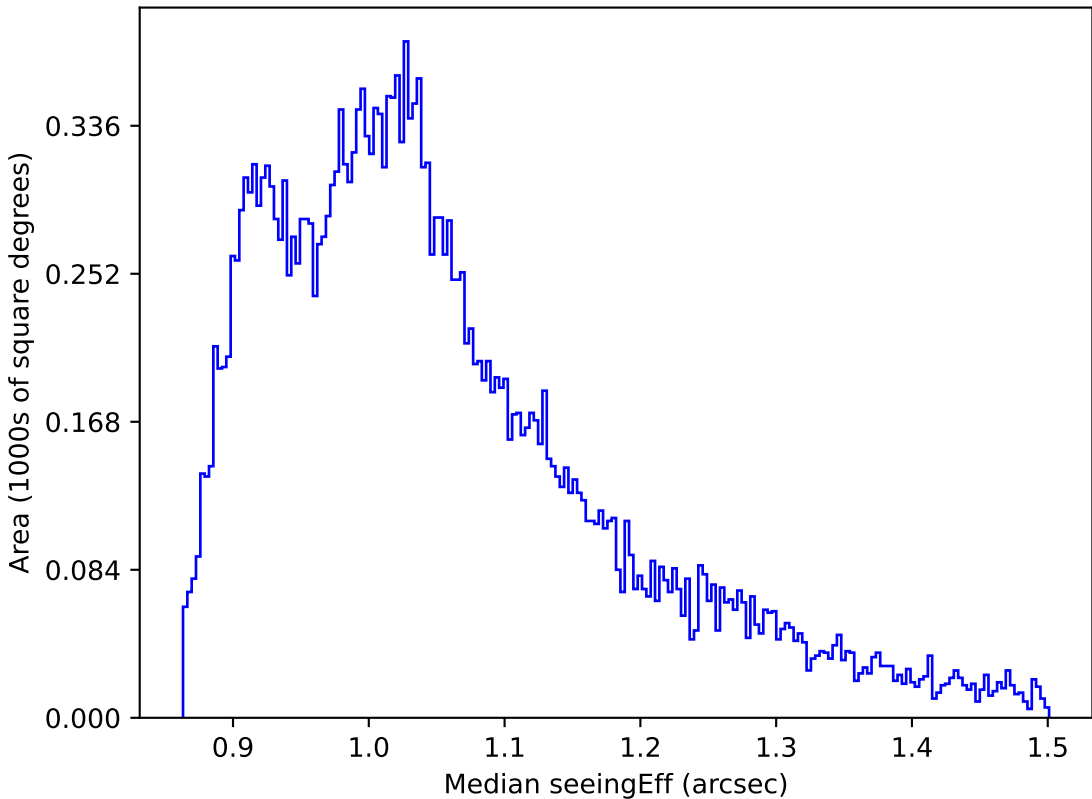
weather_cloudso31v3.4_10yrs All sky i band: Median seeingEff
