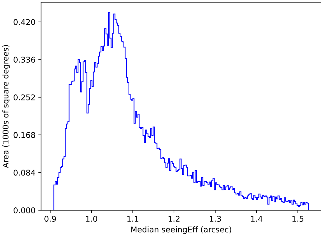
weather_cloudso31v3.4_10yrs All sky all bands: Median seeingEff
