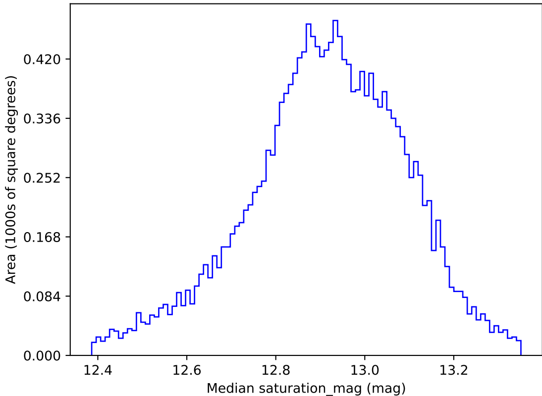
weather_cloudso31v3.4_10yrs WFD u band: Median saturation_mag
