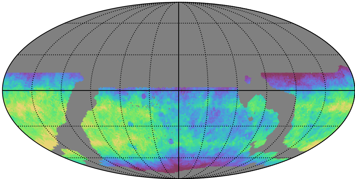
weather_cloudso31v3.4_10yrs WFD r band: Median saturation_mag
