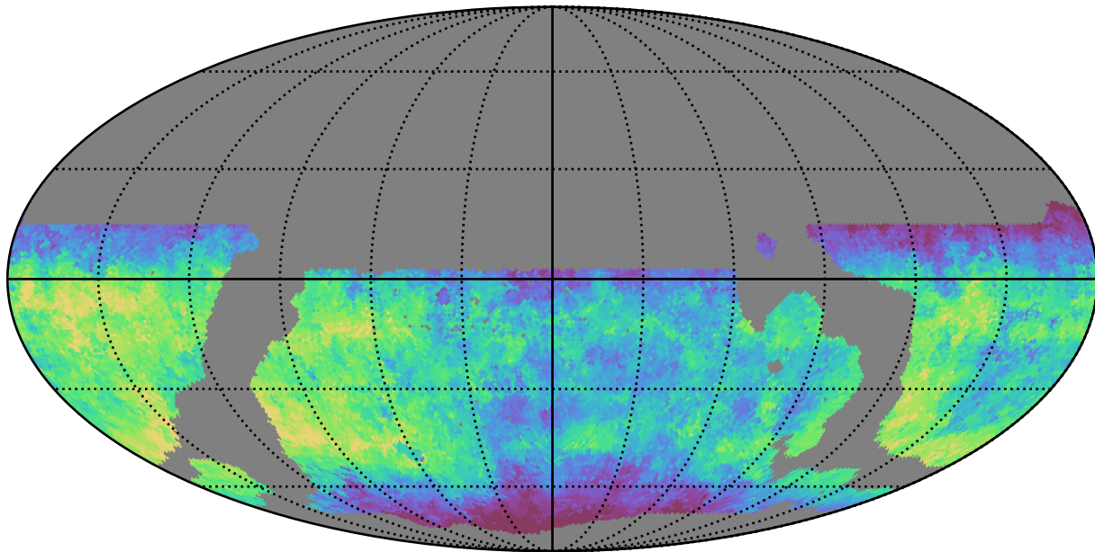
weather_cloudso31v3.4_10yrs WFD g band: Median saturation_mag
