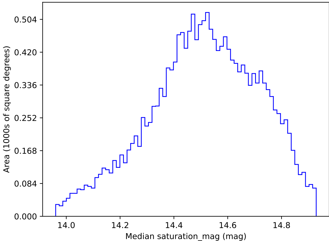
weather_cloudso31v3.4_10yrs WFD g band: Median saturation_mag
