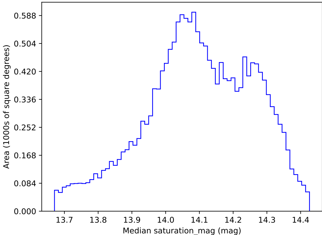
weather_cloudso31v3.4_10yrs WFD all bands: Median saturation_mag
