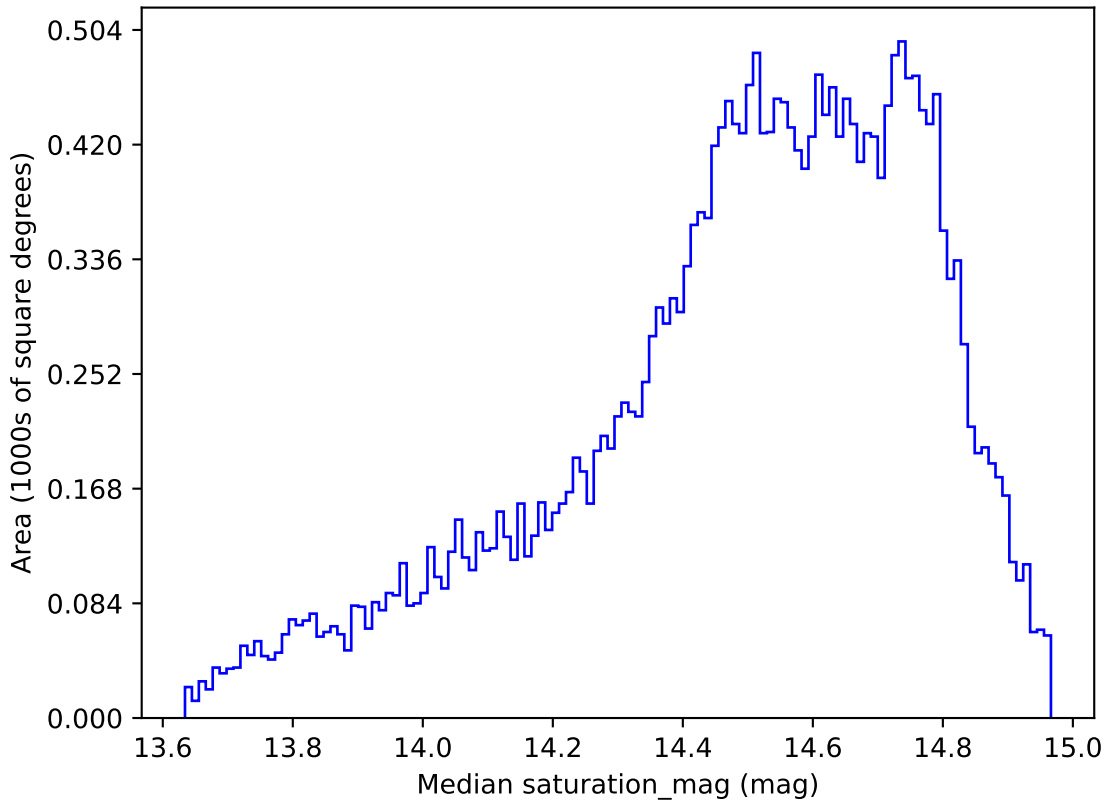
weather_cloudso31v3.4_10yrs All sky r band: Median saturation_mag
