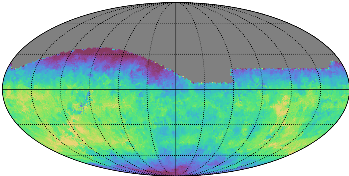
weather_cloudso31v3.4_10yrs All sky g band: Median saturation_mag
