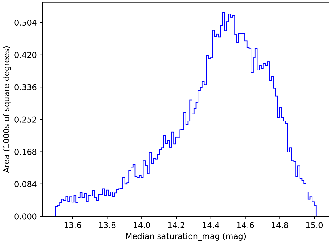
weather_cloudso31v3.4_10yrs All sky g band: Median saturation_mag
