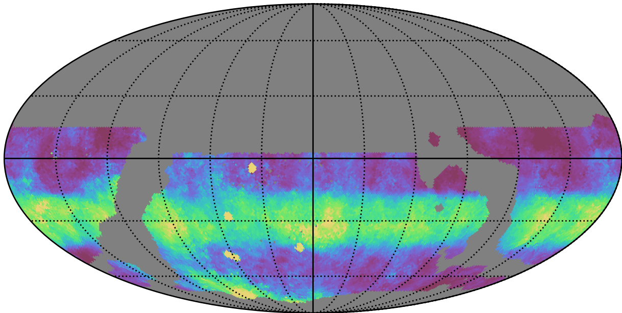
weather_cloudso31v3.4_10yrs WFD z band: Median normairmass
