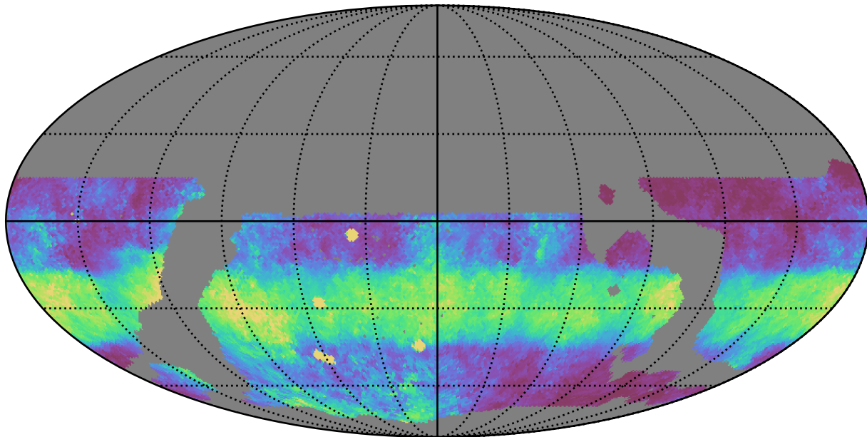
weather_cloudso31v3.4_10yrs WFD y band: Median normairmass
