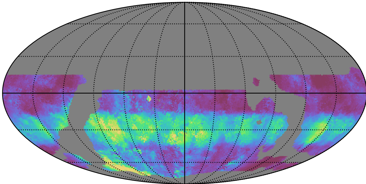
weather_cloudso31v3.4_10yrs WFD u band: Median normairmass
