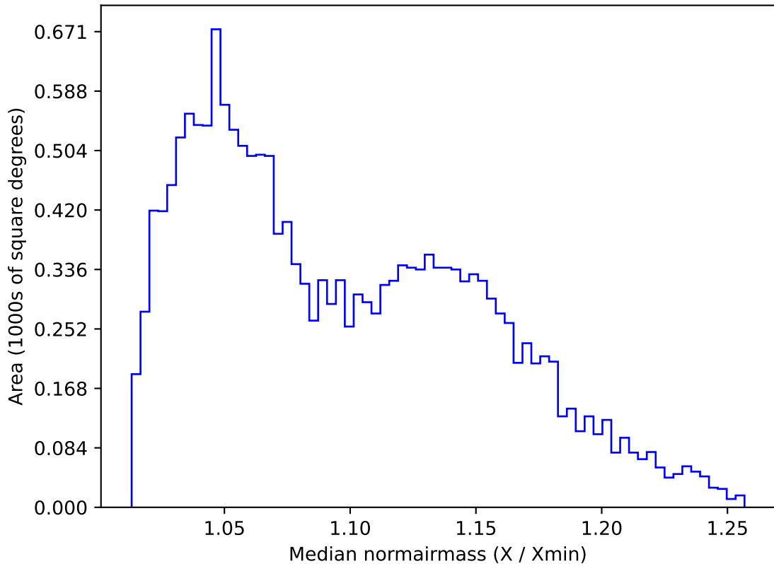
weather_cloudso31v3.4_10yrs WFD u band: Median normairmass
