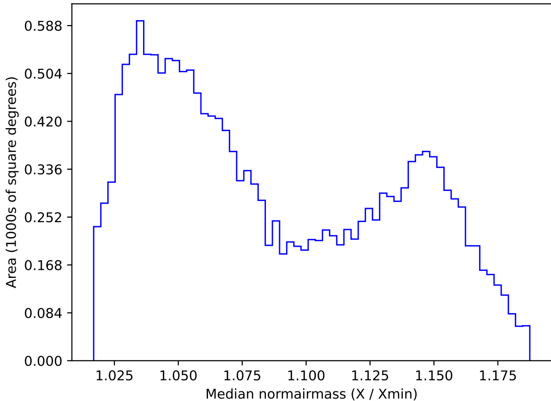
weather_cloudso31v3.4_10yrs WFD r band: Median normairmass
