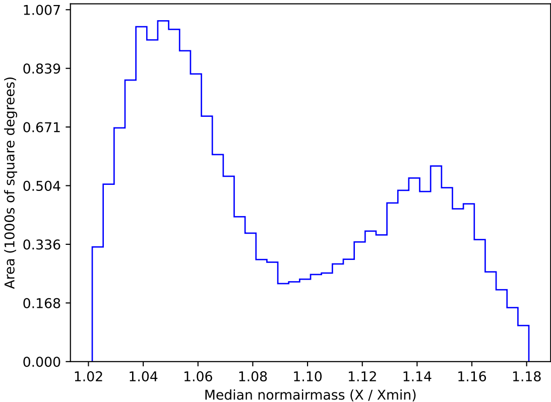
weather_cloudso31v3.4_10yrs WFD i band: Median normairmass
