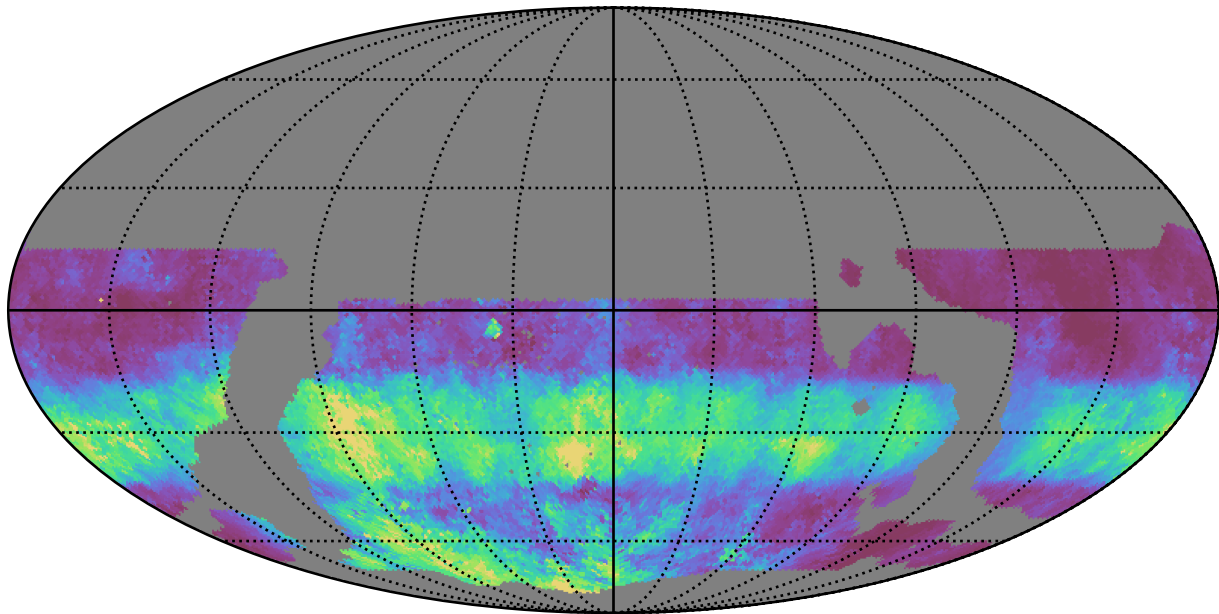
weather_cloudso31v3.4_10yrs WFD g band: Median normairmass
