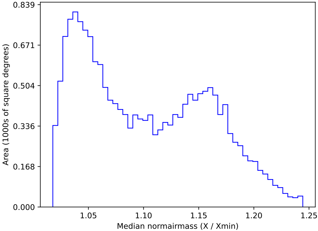
weather_cloudso31v3.4_10yrs WFD g band: Median normairmass
