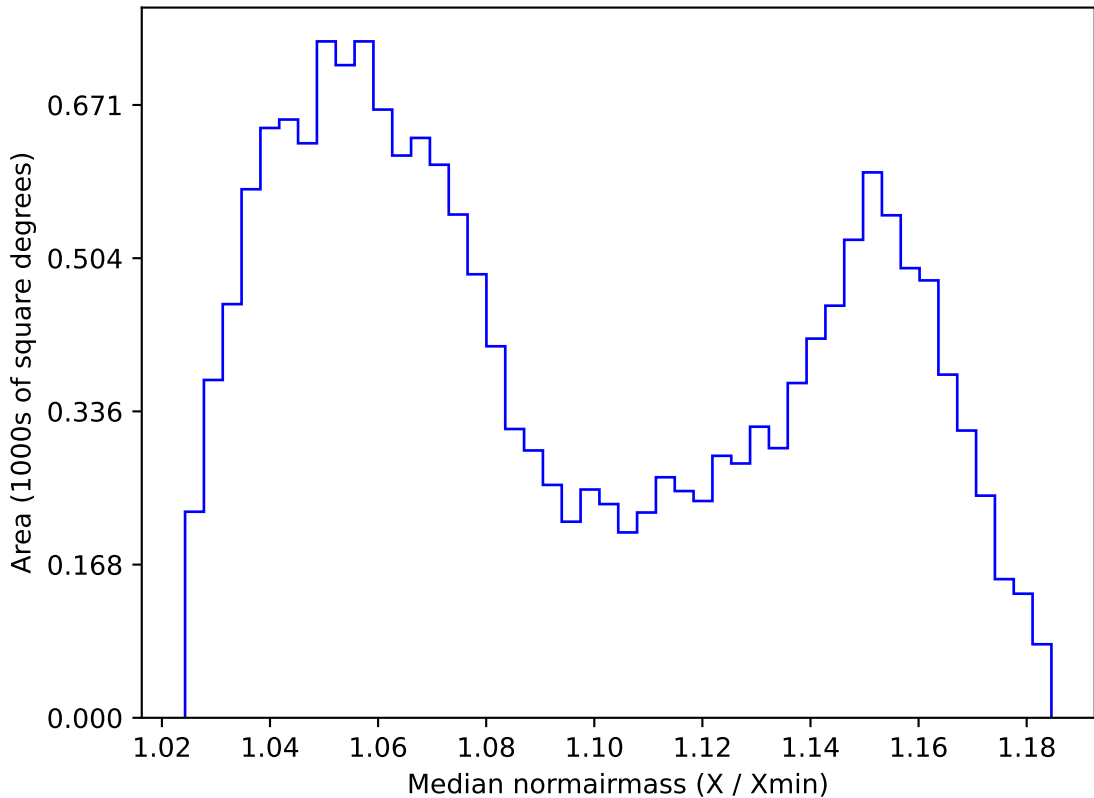
weather_cloudso31v3.4_10yrs WFD all bands: Median normairmass
