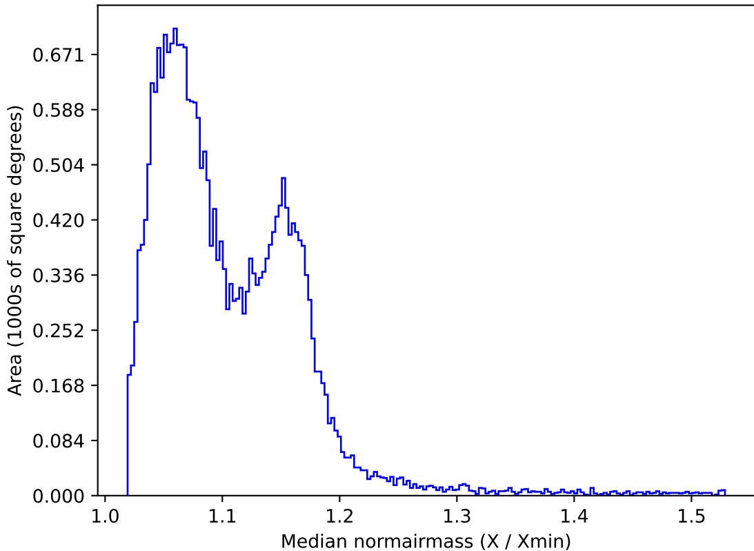
weather_cloudso31v3.4_10yrs All sky z band: Median normairmass
