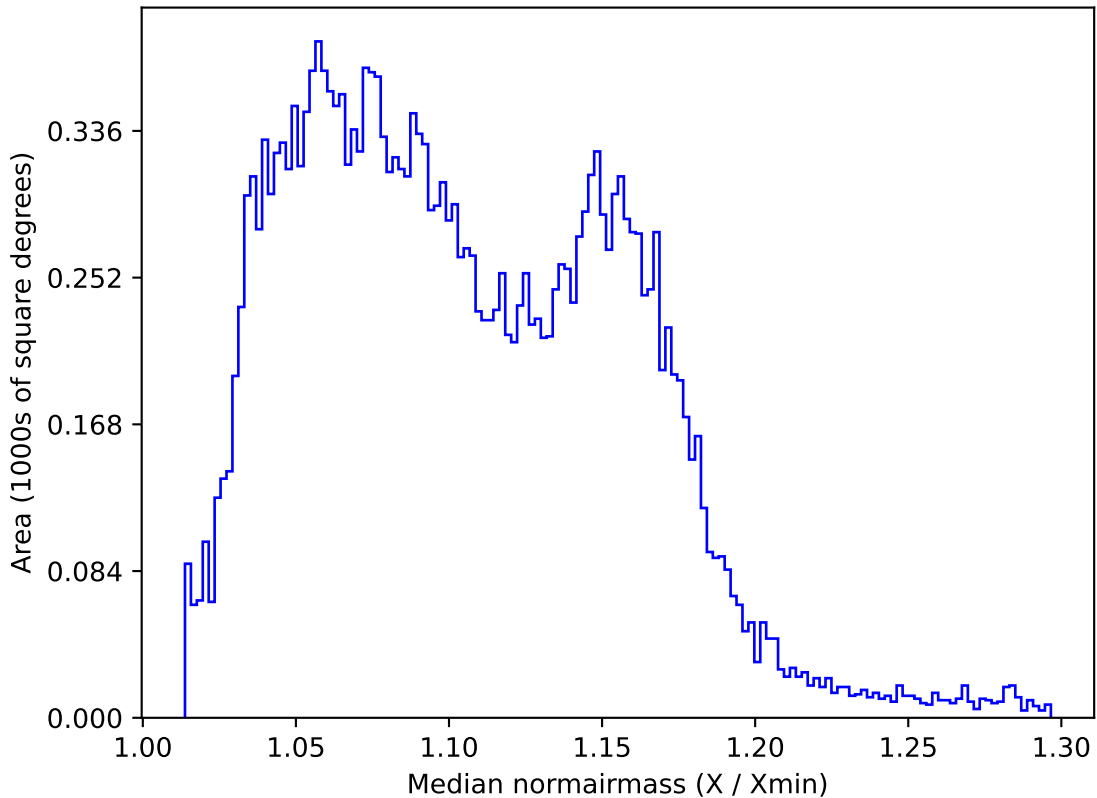
weather_cloudso31v3.4_10yrs All sky y band: Median normairmass
