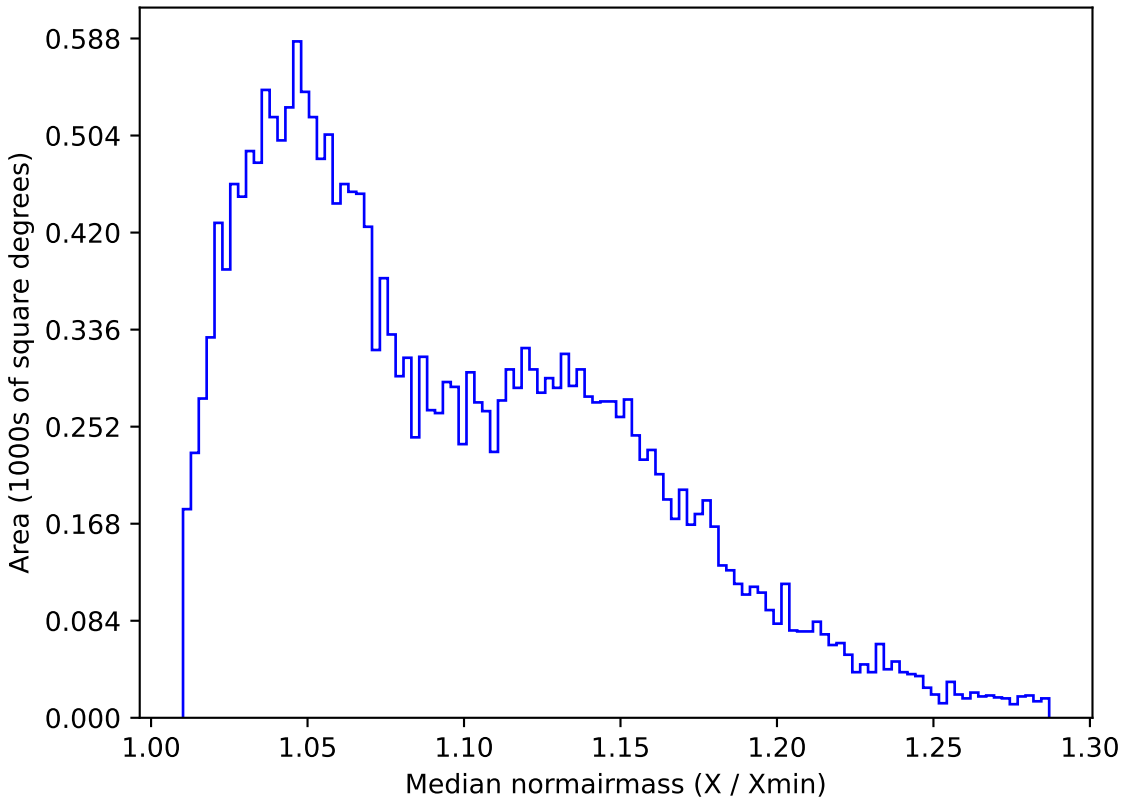
weather_cloudso31v3.4_10yrs All sky u band: Median normairmass
