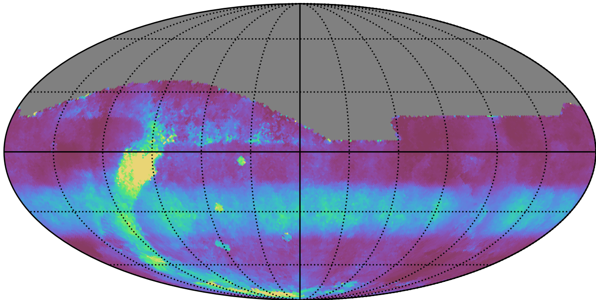
weather_cloudso31v3.4_10yrs All sky r band: Median normairmass
