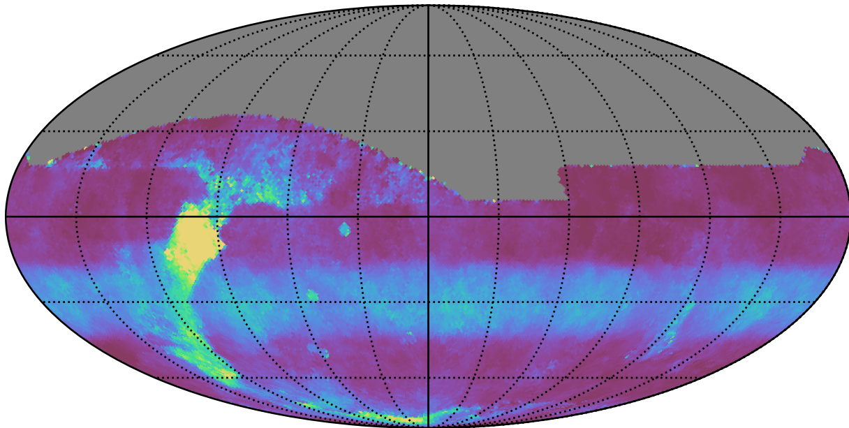
weather_cloudso31v3.4_10yrs All sky i band: Median normairmass
