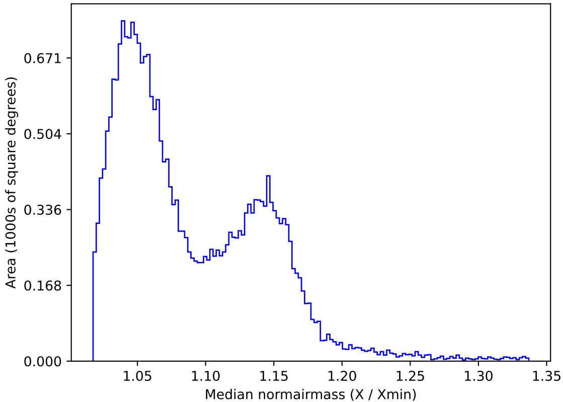
weather_cloudso31v3.4_10yrs All sky i band: Median normairmass
