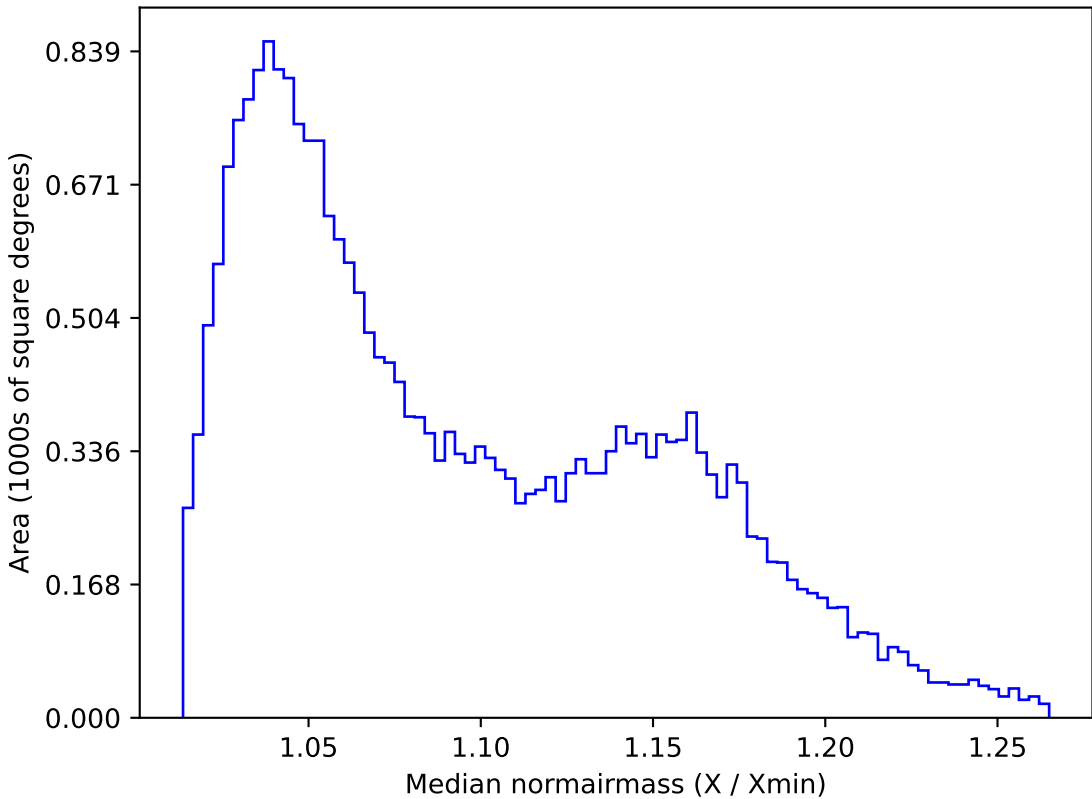
weather_cloudso31v3.4_10yrs All sky g band: Median normairmass
