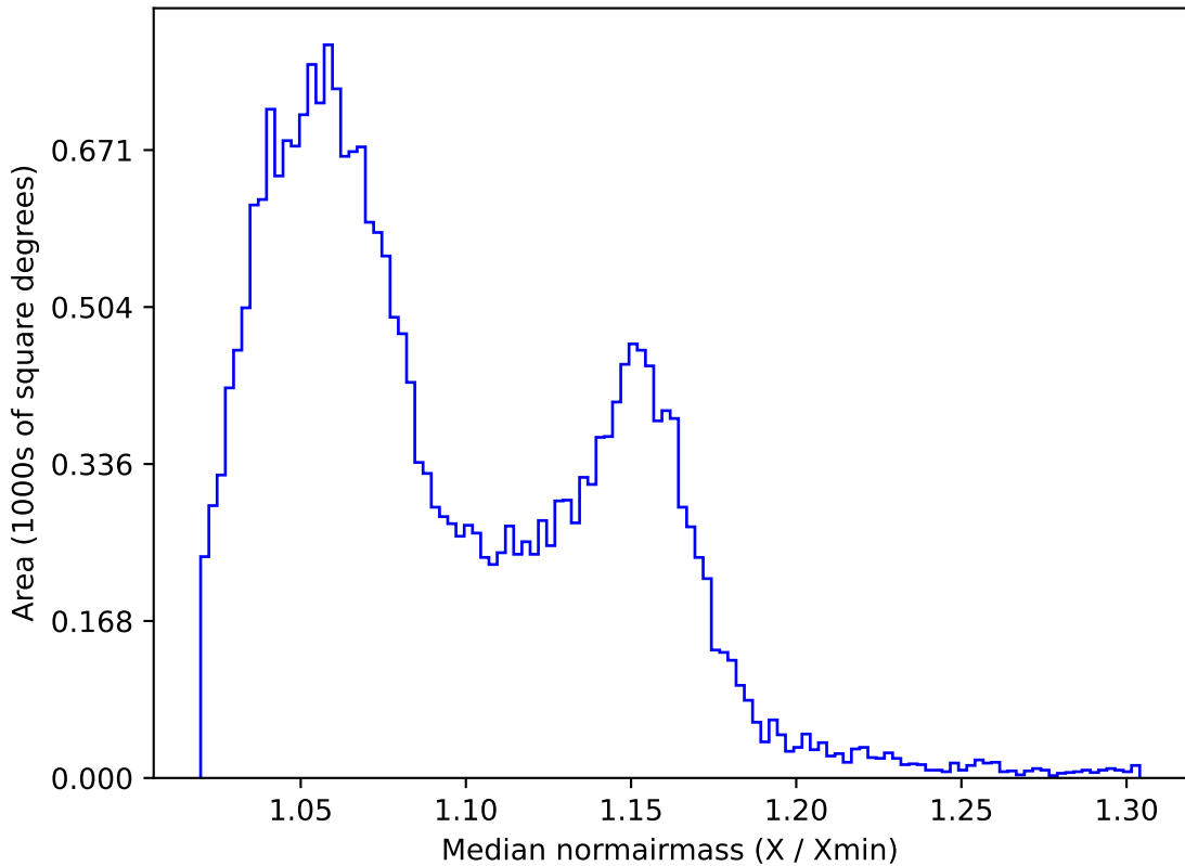
weather_cloudso31v3.4_10yrs All sky all bands: Median normairmass
