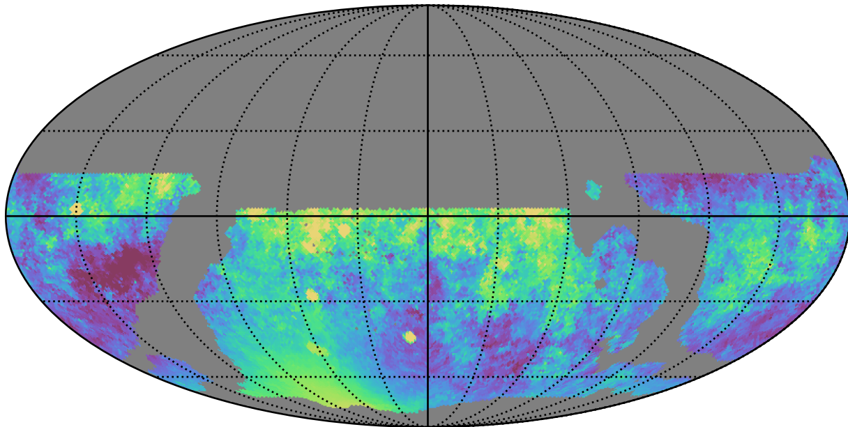
weather_cloudso31v3.4_10yrs WFD z band: Median moonDistance
