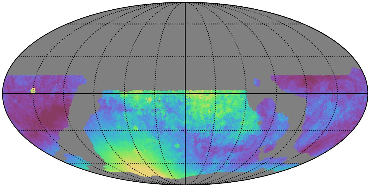
weather_cloudso31v3.4_10yrs WFD y band: Median moonDistance
