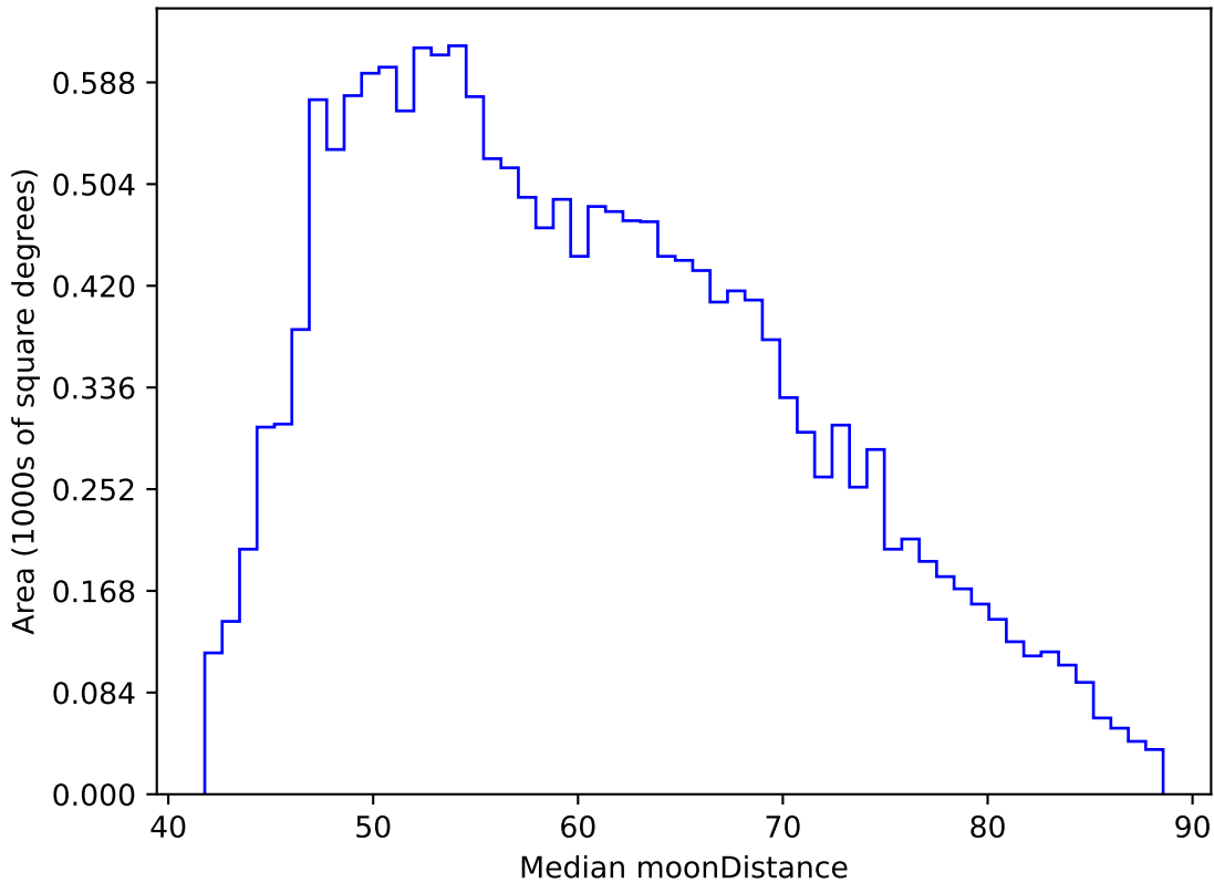
weather_cloudso31v3.4_10yrs WFD y band: Median moonDistance
