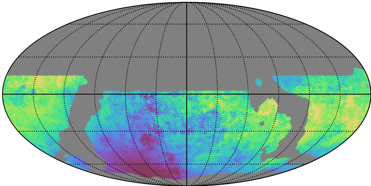
weather_cloudso31v3.4_10yrs WFD u band: Median moonDistance
