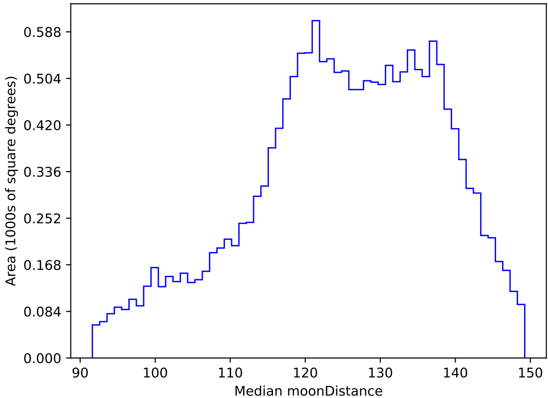
weather_cloudso31v3.4_10yrs WFD u band: Median moonDistance
