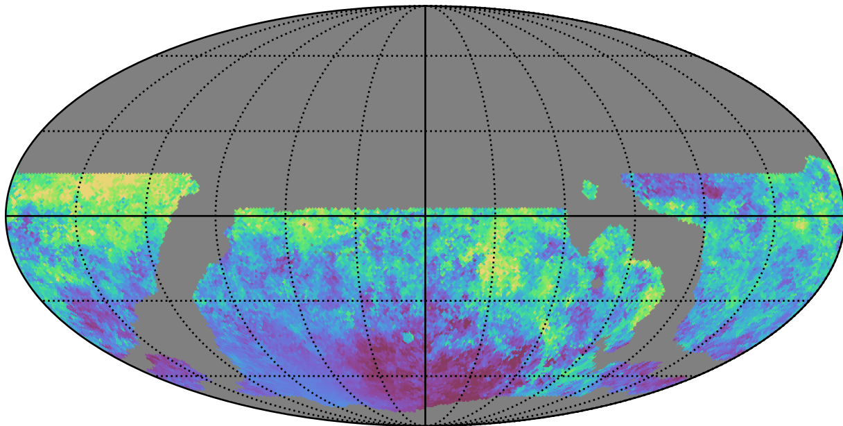
weather_cloudso31v3.4_10yrs WFD i band: Median moonDistance
