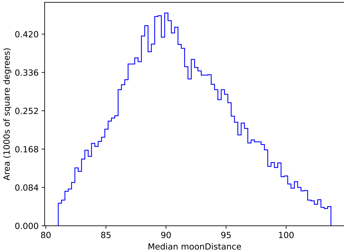
weather_cloudso31v3.4_10yrs WFD all bands: Median moonDistance
