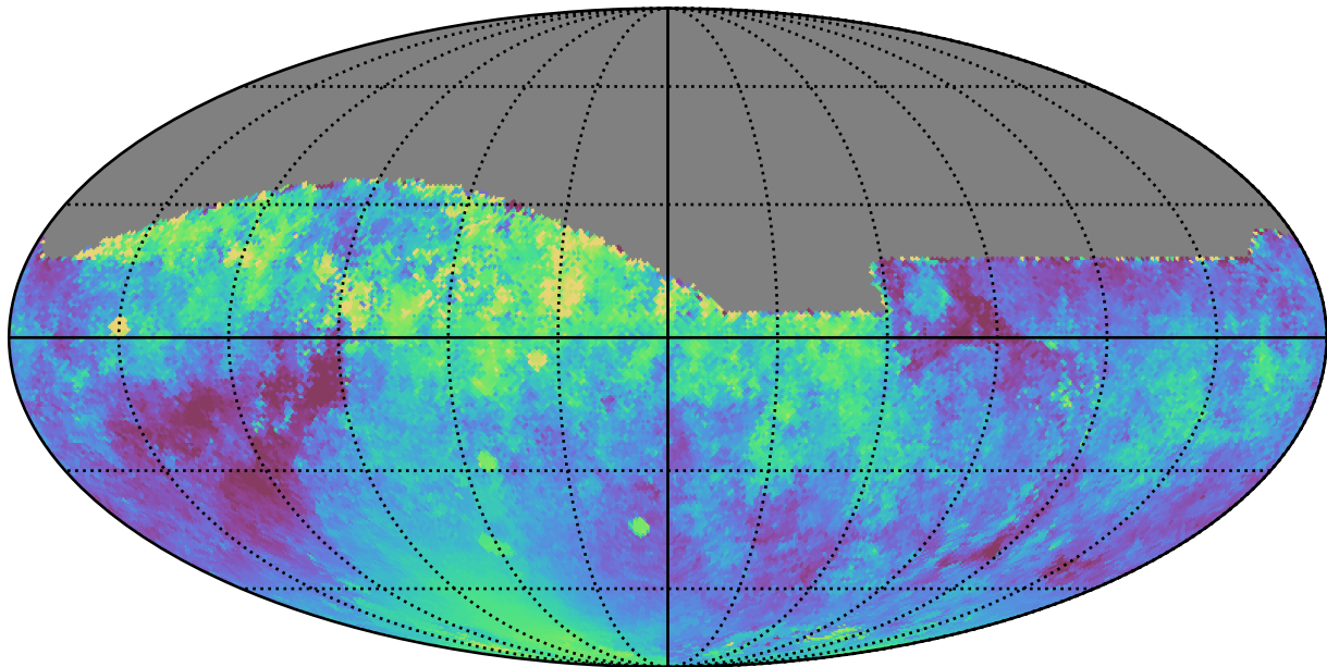
weather_cloudso31v3.4_10yrs All sky z band: Median moonDistance
