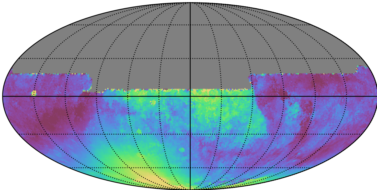
weather_cloudso31v3.4_10yrs All sky y band: Median moonDistance
