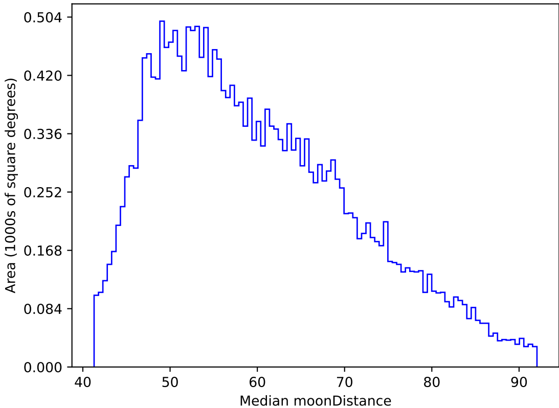
weather_cloudso31v3.4_10yrs All sky y band: Median moonDistance
