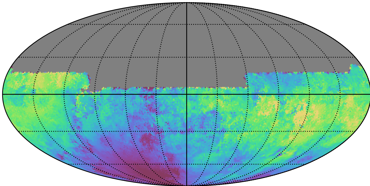
weather_cloudso31v3.4_10yrs All sky u band: Median moonDistance
