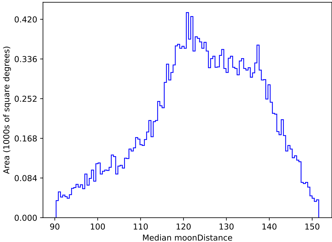
weather_cloudso31v3.4_10yrs All sky u band: Median moonDistance
