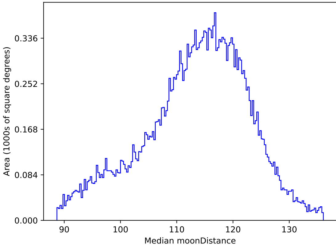
weather_cloudso31v3.4_10yrs All sky r band: Median moonDistance
