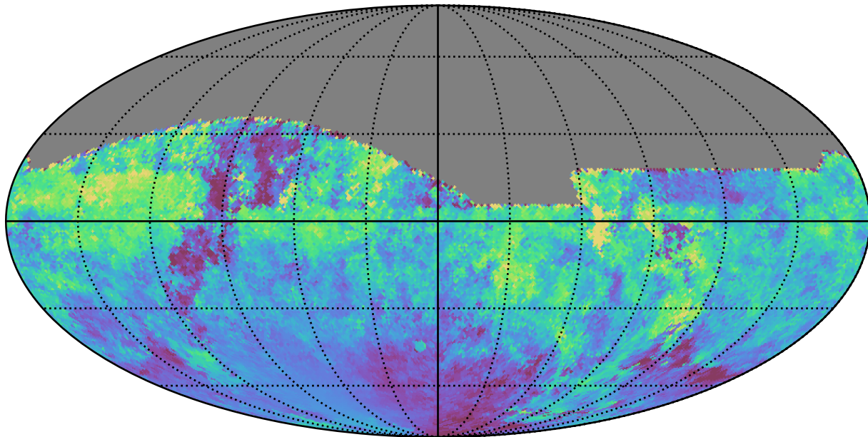
weather_cloudso31v3.4_10yrs All sky i band: Median moonDistance
