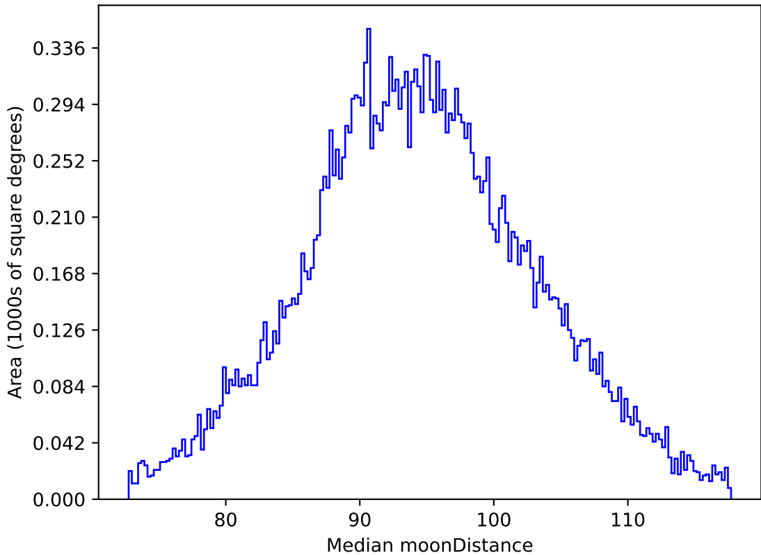
weather_cloudso31v3.4_10yrs All sky i band: Median moonDistance
