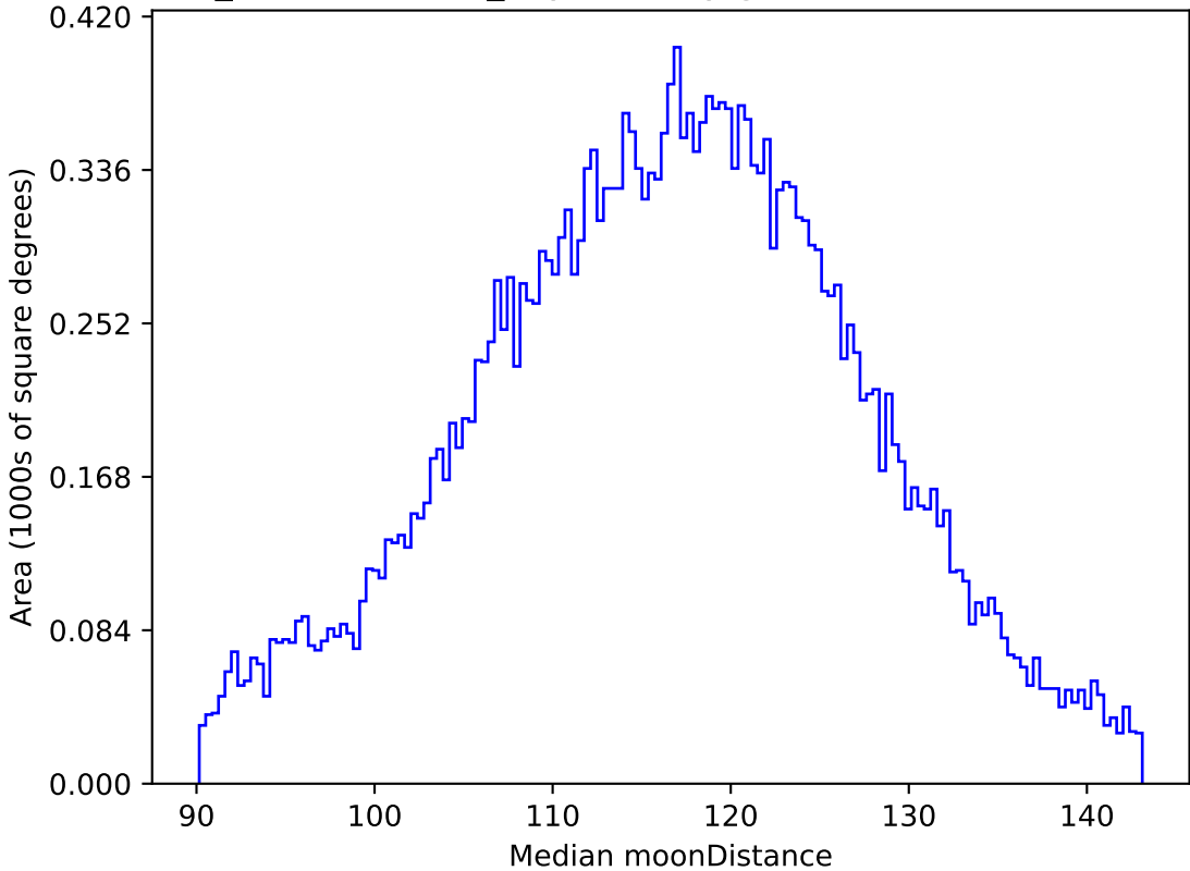
weather_cloudso31v3.4_10yrs All sky g band: Median moonDistance
