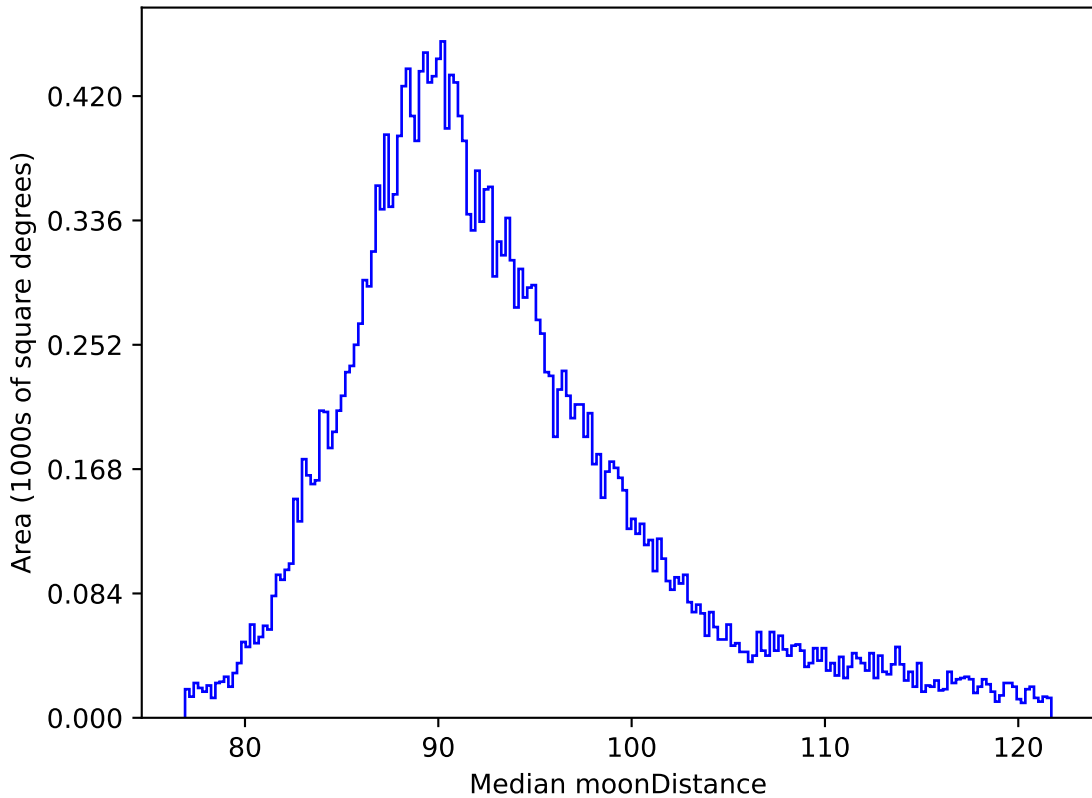
weather_cloudso31v3.4_10yrs All sky all bands: Median moonDistance
