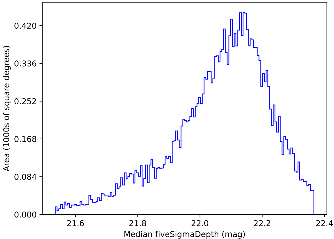
weather_cloudso31v3.4_10yrs Yr 1 y band: Median fiveSigmaDepth
