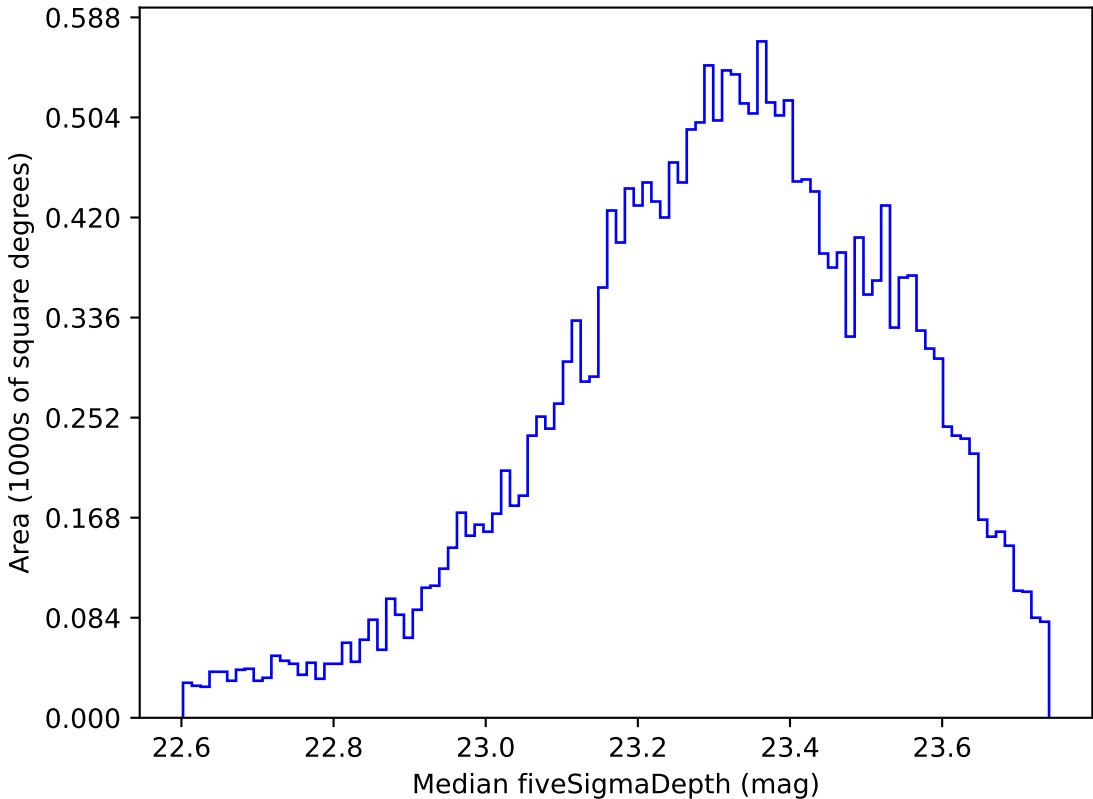
weather_cloudso31v3.4_10yrs Yr 1 u band: Median fiveSigmaDepth
